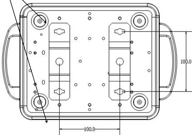
Rubber feet for floor mounting*4
